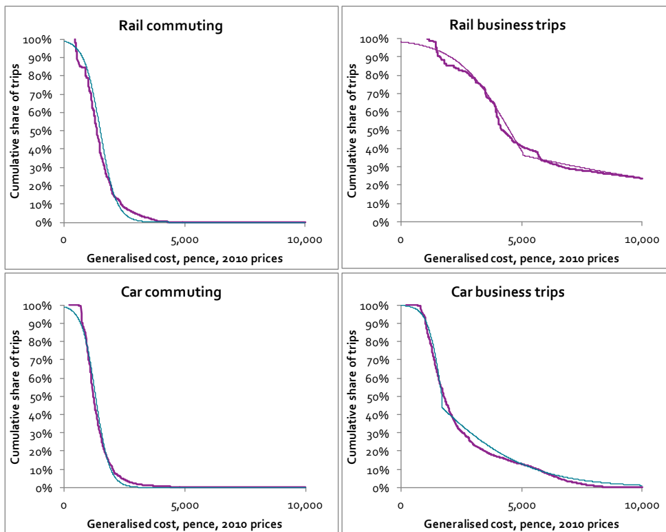
Figure 18: Decay curves derived for rail and car trips by journey purpose (2010)
